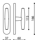
C185R - fixed window slider
