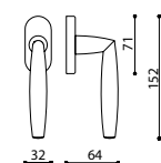
K185R - operational window handle
